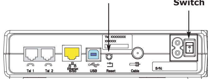
Reset Button
